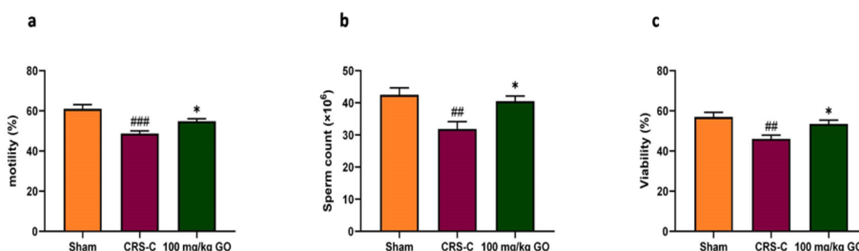
Figure 5. Effects of GO on sperm parameters in experimental groups after restraint stress exposure. (a) Percentage of sperm motility, (b) Sperm counts, and (c) Percentage of sperm viability. The data are presented as mean±SEM (N=8). ##p<0.01 and ###p<0.001 vs. the sham group. *p<0.05 vs. the CRS-C group. CRS-C: chronic restraint stress control; GO: gamma oryzanol
