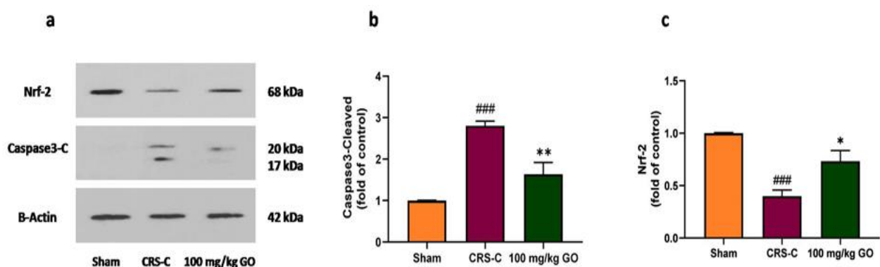
Figure 7. Effects of GO on protein expression in the testicular tissues of experimental groups after restraint stress exposure. (a) Representative images of protein expressions investigated by western blotting, (b) Caspase 3-cleaved, and (c) Nrf-2. The data are shown as mean \pm SEM (N=3). ### p<0.001 vs. the sham group. * p<0.05 and ** p<0.01 vs. the CRS-C group. CRS-C: chronic restraint stress control; GO: gamma oryzanol
