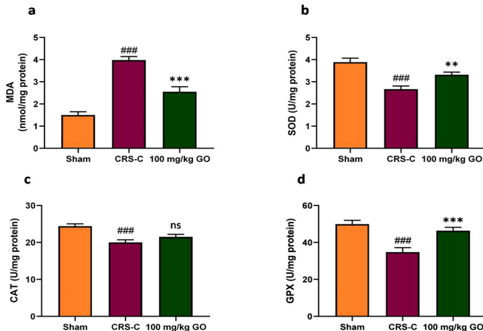
Figure 6. Effects of GO on the antioxidant levels of testicular tissue in the experimental groups after restraint stress exposure. (a) MDA, (b) SOD, (c) CAT, and (d) GPx. The data are shown as mean \pm SEM (N=8). ### p<0.001 vs. the sham group. ** p<0.01 and *** p<0.001 vs. the CRS-C group. CRS-C: chronic restraint stress control; GO: gamma oryzanol; ns: non-significant
