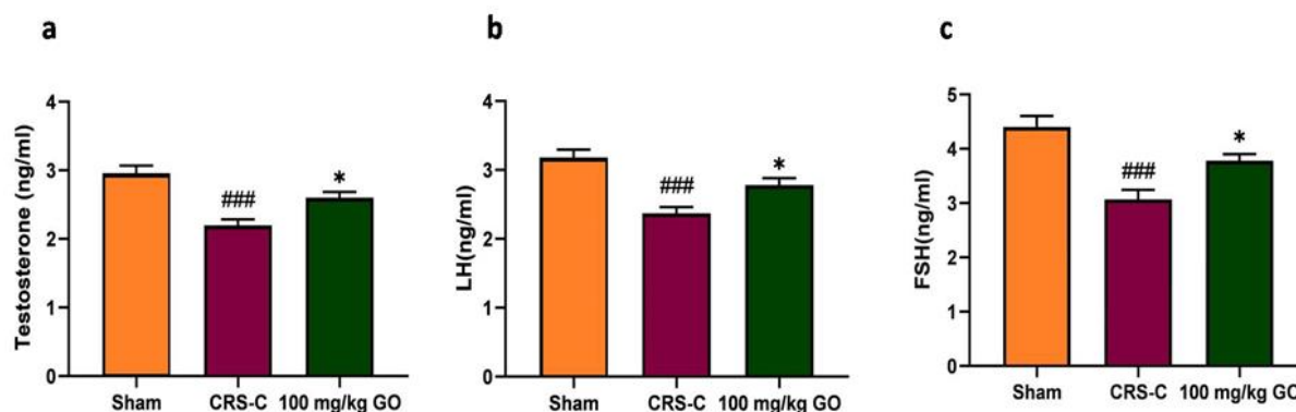
Figure 4. Effects of GO on the reproductive hormone levels in the experimental groups after restraint stress exposure. (a) Testosterone, (b) LH, and c. FSH. The data are shown as mean±SEM (N=8). ###p<0.001 vs. the sham group. *p<0.05 vs. the CRS-C group. CRS-C: chronic restraint stress control; GO: gamma oryzanol
